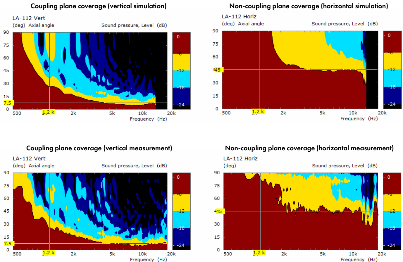
Figure 5. Simulated and measured coverage contour plots of the LA112 loudspeaker's waveguide at a distance of 4 m (13 ft).
