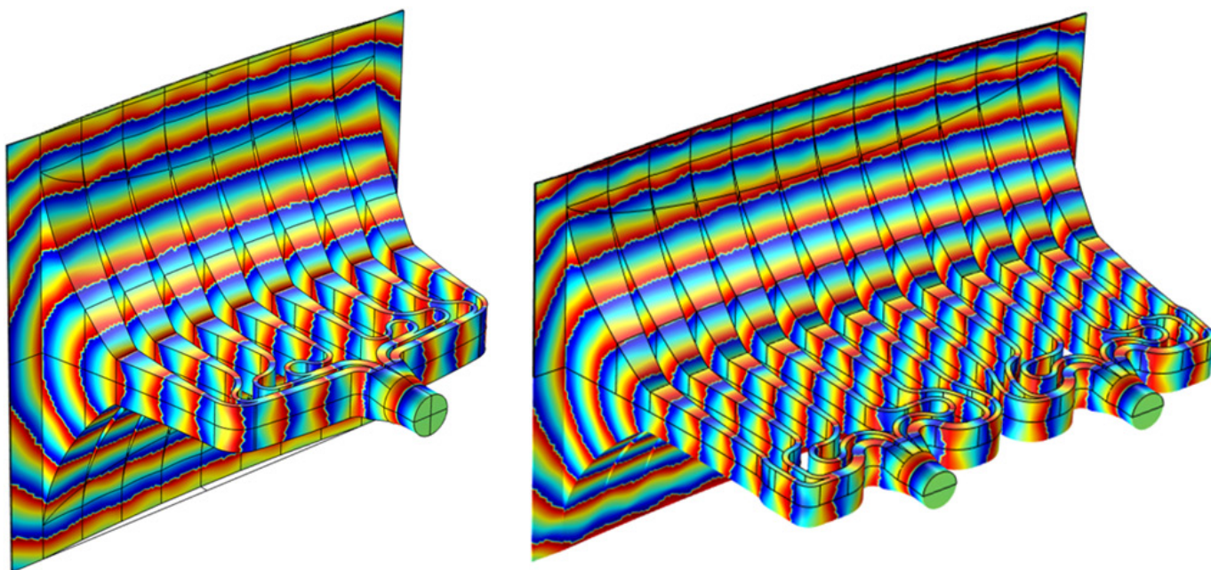
Figure 3. Isometric views depicting phase analysis within LA108 (left) and LA112 (right) waveguides at 15 kHz.
