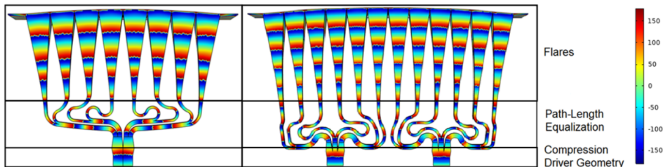
Figure 2. Phase analysis inside LA108 (left) and LA112 (right) waveguides at 15 kHz in a cross-section within the coupling plane.
