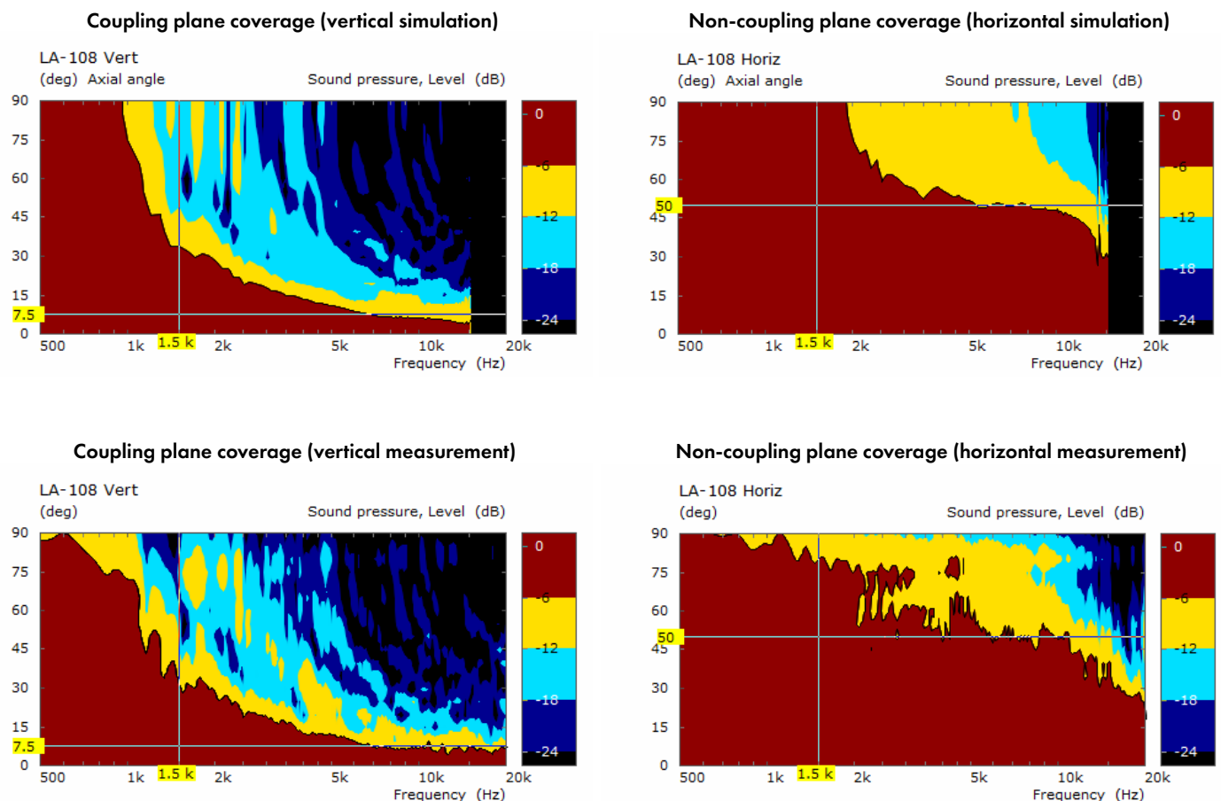
Figure 4. Simulated and measured coverage contour plots of the LA108 loudspeaker’s waveguide at a distance of 4 m (13 ft).
