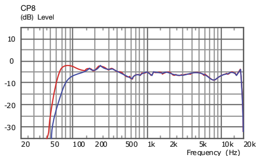
CP8 On-Axis Frequency Response
