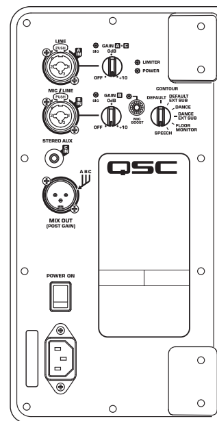
CP8 / CP12 Back Panel
