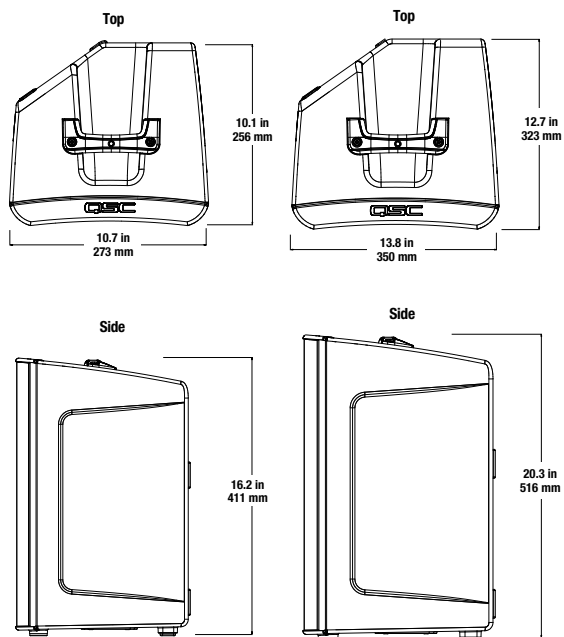
CP8 / CP12 Top and Side
