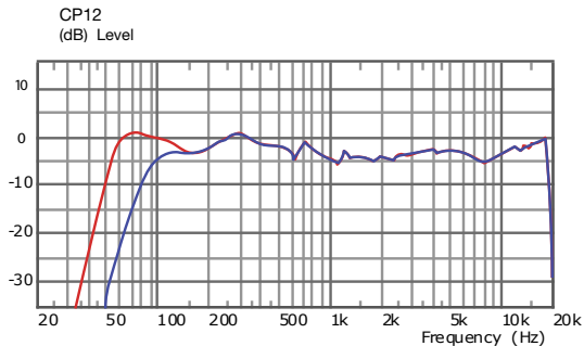
CP12 On-Axis Frequency Response
