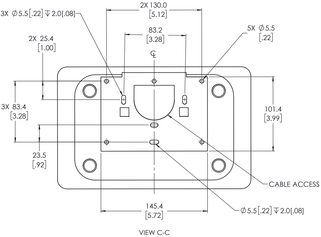
VIEW C-C
