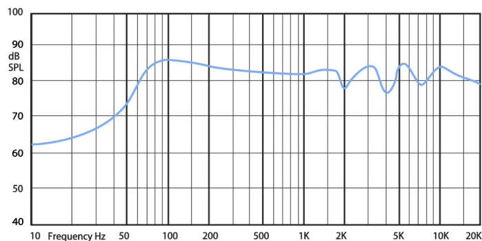
Frequency response
