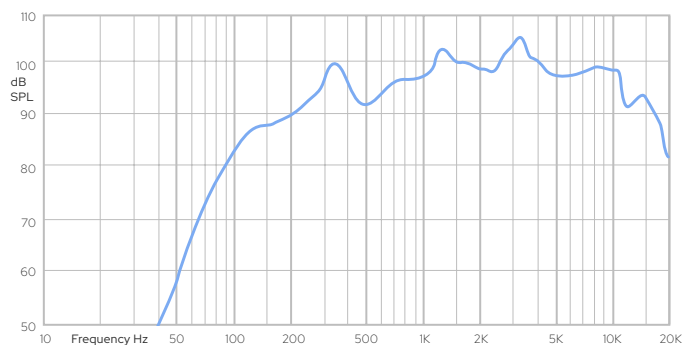
Frequency response
