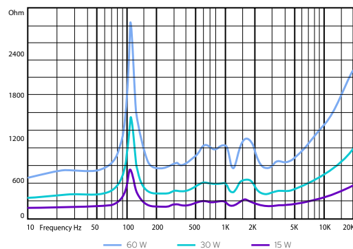
Impedance
