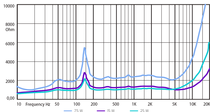
Impedance
