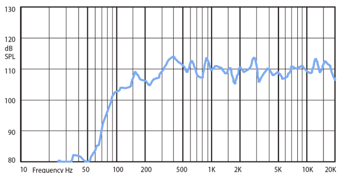
Frequency response
