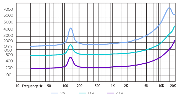
Impedance
