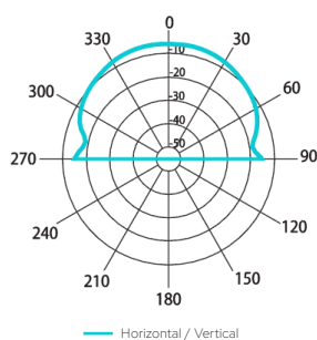
Horizontal/vertical polar diagrams
