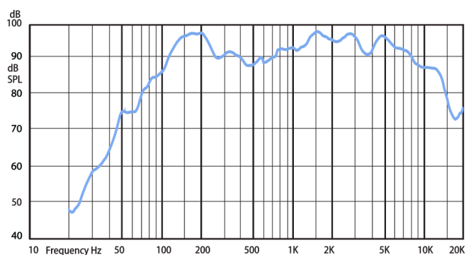
Frequency response
