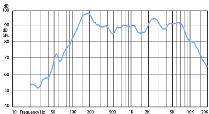
Frequency response
