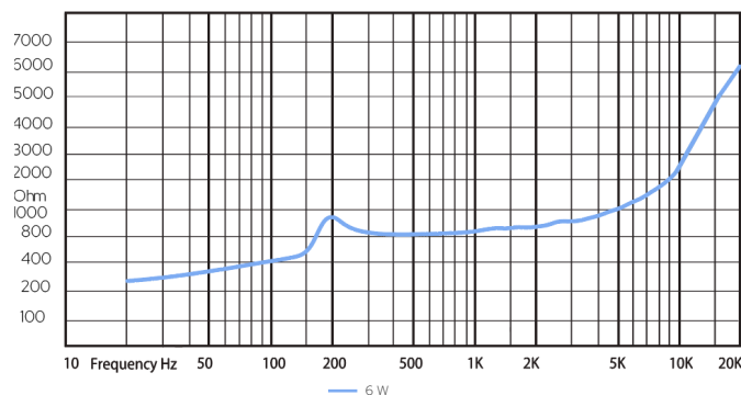
Impedance
