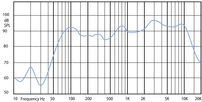
Frequency response
