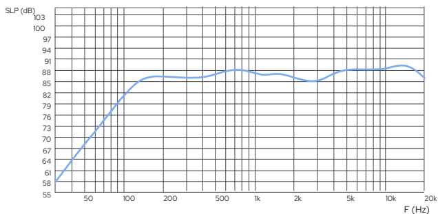
Frequency response 04 LOUDSPEAKER
